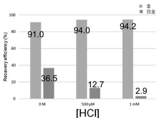
図5 上澄み液の ICP (monoAntED)
