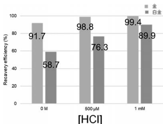
図4 上澄み液の ICP (diAntED)
